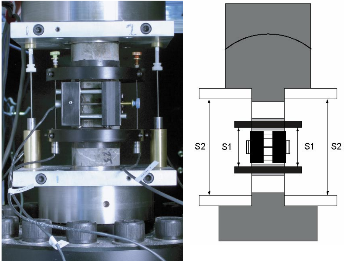
Figure 3-3. Left: Specimen inserted between the loading platens. The two separate axial deformation measurement devices can be seen: system (S1) that measures the local axial deformation (rings) and system (S2) that measures the deformation between the aluminium plates (total deformation). Right: Principal sketch showing the two systems used for the axial deformation measurements.
