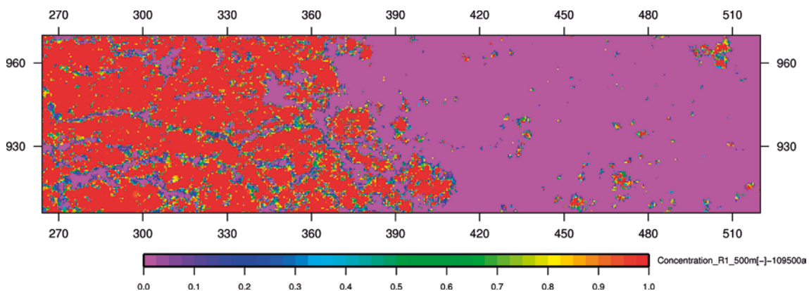
Figure 7-12. Case 1: glacial meltwater concentration (expressed in mass fraction [-] ) at -110 ka, after 500 years of transport, period of glacial build up , projected horizontal cut at 500 meter depth (coordinates in km).
