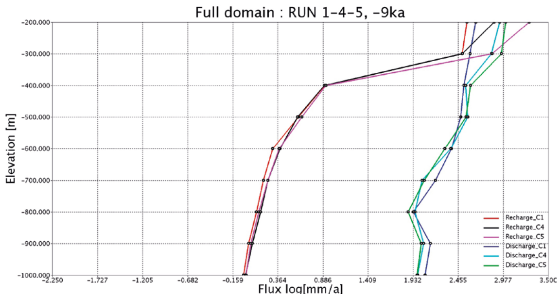
Figure 7-6. Cases 1, 4 and 5 at -9 ka, period of glacial retreat (with apparition of ice margin), average recharge/ discharge, \log[\text{mm/a}] , in terms of elevation, for the modelled domain.
