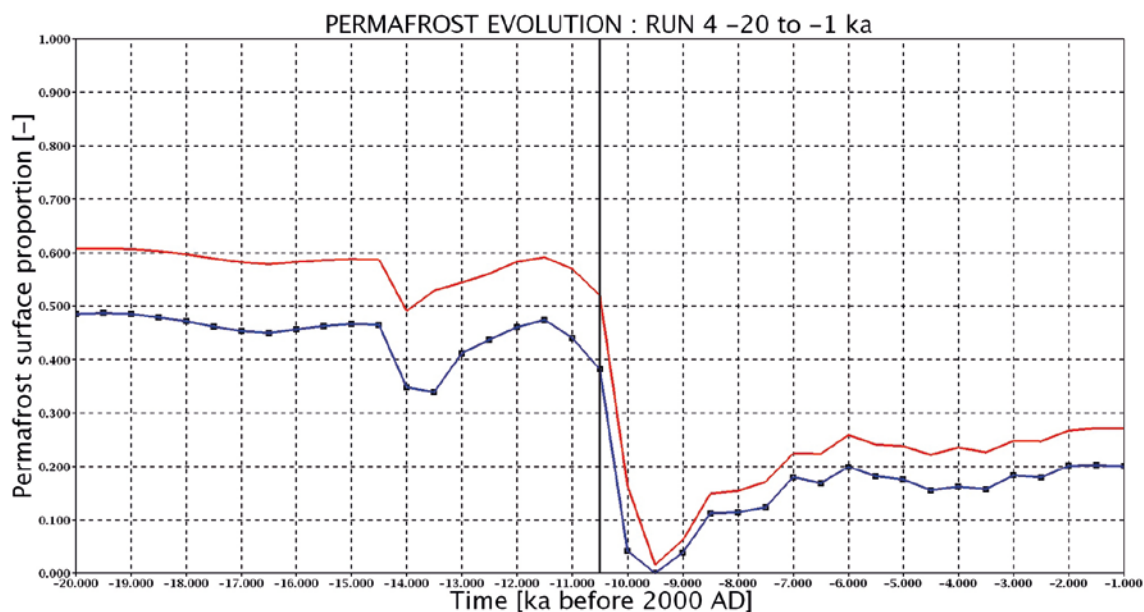
Figure 6-69. Case 4: evolution of permafrost proportion [-] over the model surface (blue line) in comparison to the case 1 (red line) from -20 to -1 ka. The onset of glacial retreat is at -10.5 ka (vertical black line). The lowest value of permafrost proportion during glacial retreat occurs at -9.5 ka. From -9.5 to -1 ka, the permafrost is no longer present under the ice sheet.
