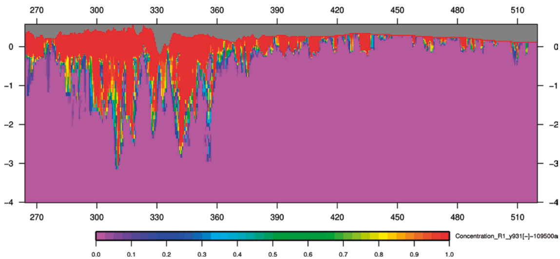
Figure 7-11. Case 1: glacial meltwater concentration (expressed in mass fraction [-] ), at -110 ka, after 500 years of transport, period of glacial build up , E-W vertical at Y = 931 km (coordinates in km).
