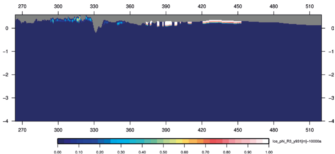
Figure 6-54. Case 3: permafrost (white) at -10 ka (expressed as ice proportion [-]), period of glacial retreat , E-W vertical at Y = 931 km (coordinates in km).
