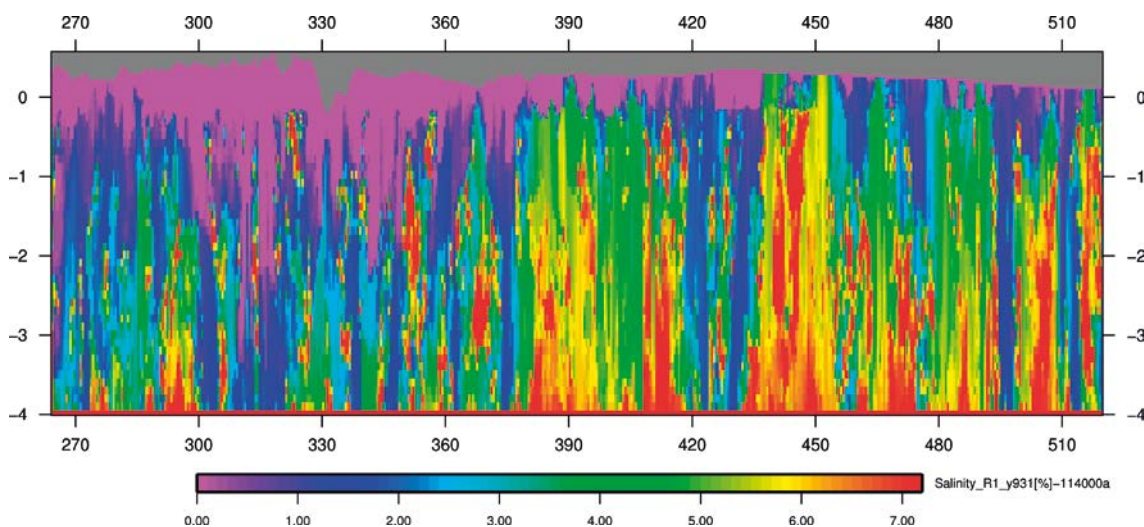
Figure 6-32. Case 1: salinity [%] at -114 ka with the absence of ice sheet , E-W vertical at Y = 931 km (coordinates in km).
