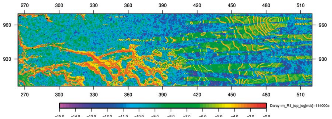
Figure 6-39. Case 1: Darcy velocity module, \log[m/s] at -114 ka with the absence of ice sheet , projected top horizontal cut (coordinates in km).
