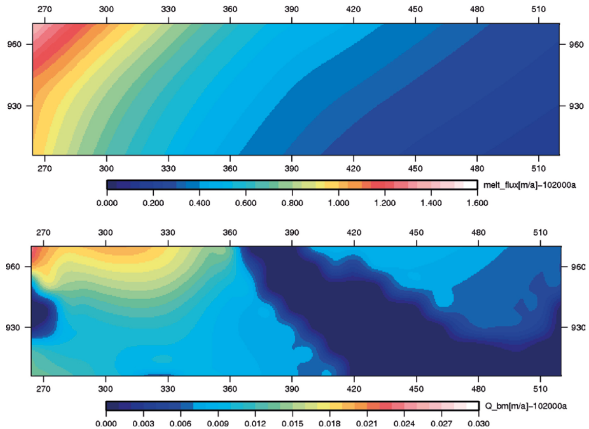
Figure C-2. Period of glacial completeness ( -102 ka): surface meltwater rate (above) and basal meltwater rate (below), interpolated from the SICOPOLIS ice sheet model and expressed in [m/a]; coordinates in km.
