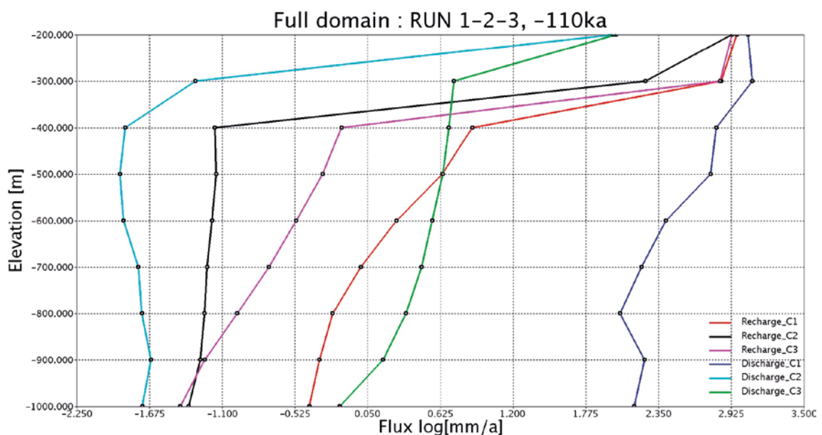
Figure 7-1. Cases 1, 2 and 3 at -110 ka, period of glacial build up , average recharge/ discharge, \log[\text{mm/a}] , in terms of elevation for the modelled domain.
