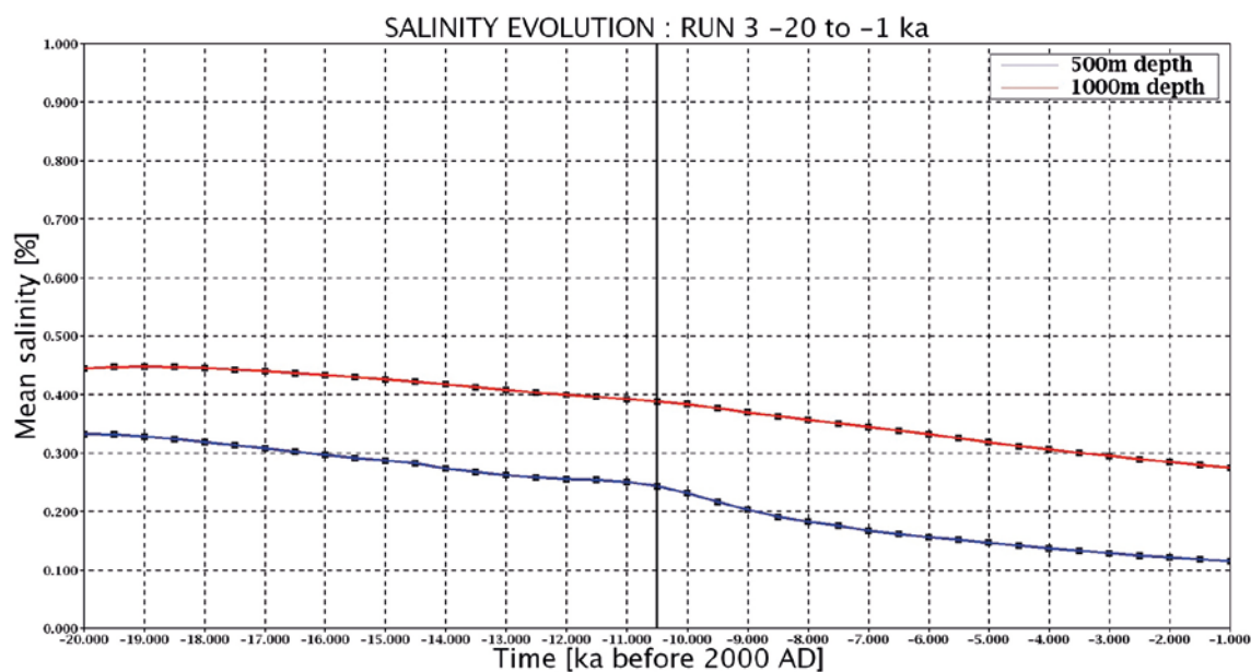
Figure 6-56. Case 3: evolution of mean salinity [%] at 500 and 1000 meter depth over the model domain, from -20 to -1ka. The onset of glacial retreat is at -10.5 ka (vertical black line).
