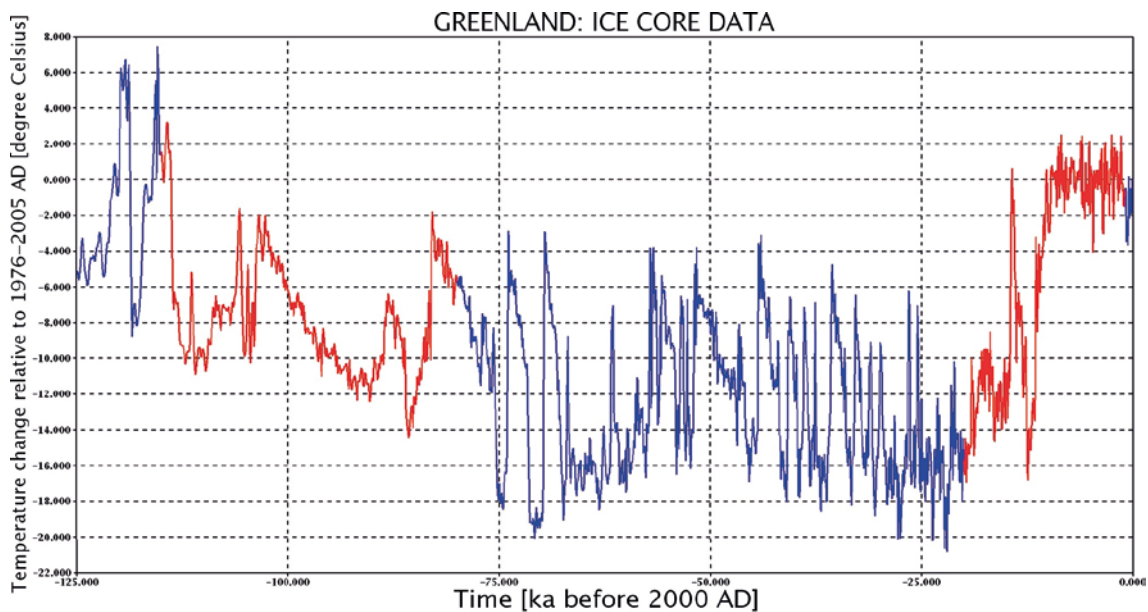
Figure 6-4. Ice core data from central-Greenland: the temperature curves for the modelled periods (–115 to –80 ka; –20 to –1 ka) are in red colour. Temperature [°C] change is relative to the mean annual 1976–2005 AD temperature.
