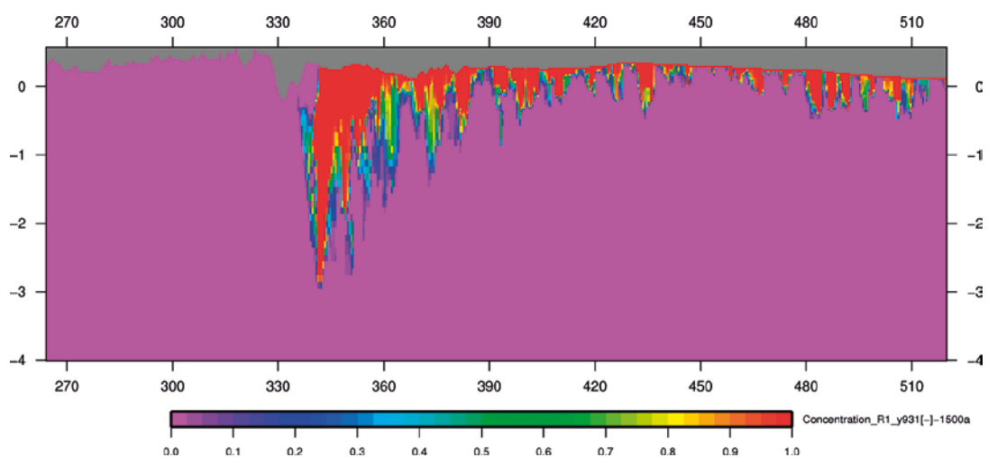
Figure 7-15. Case 1: glacial meltwater concentration (expressed in mass fraction [-]), at -2 ka, after 500 years of transport, period of glacial retreat , E-W vertical at Y = 931 km (coordinates in km).
