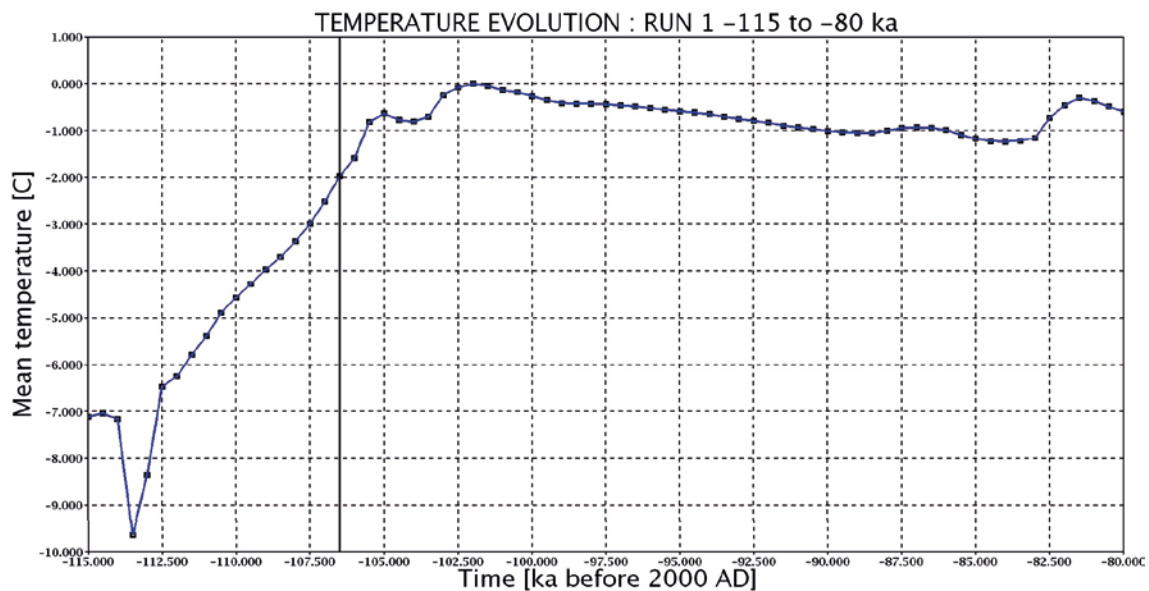
Figure 6-17. Case 1: evolution of mean temperature [ ^{\circ}\text{C} ] over the model surface, from -115 to -80 ka. The end of glacial build up is at -106.5 ka (vertical black line).
