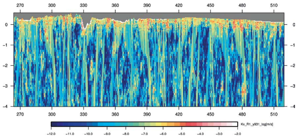
Figure 5-14. Laxemar : stochastic simulation of log-conductivity field (white represents the suglacial layer; located at the top, with K_x = 10^{-2} m/s), W-E vertical cut at Y = 931 km (coordinates in km).
