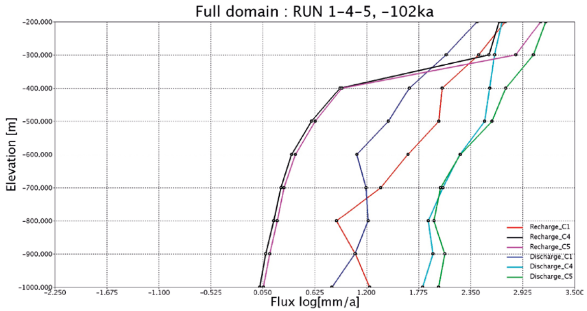
Figure 7-5. Cases 1, 4 and 5 at -102 ka, period of glacial completeness , average recharge/ discharge, \log[\text{mm/a}] , in terms of elevation, for the modelled domain.
